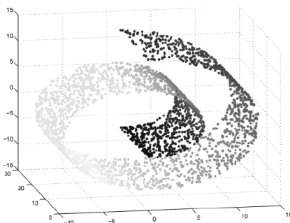
Figure 1: A curled plane: the swiss roll.
